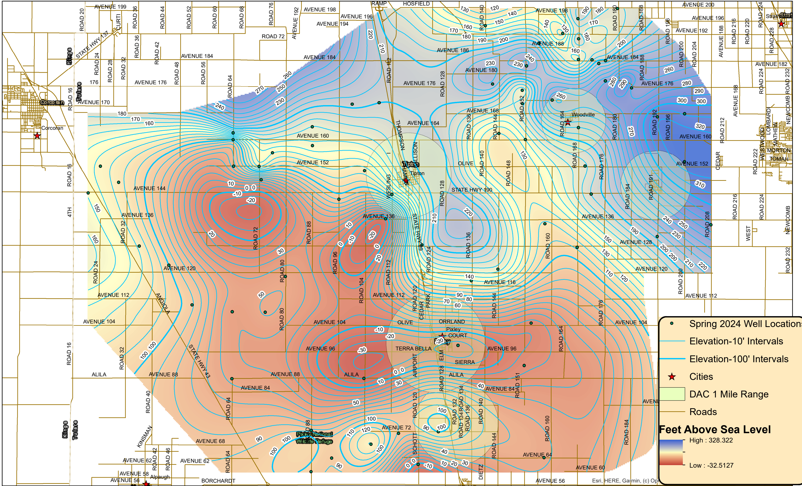
Water Surface Elevation Spring 2024
